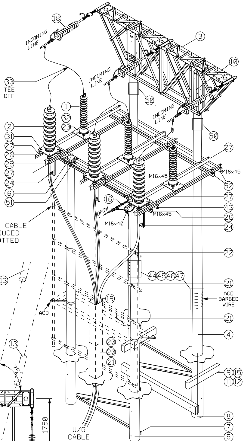
ISOMETRIC VIEW
