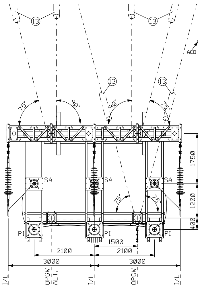
PLAN VIEW
